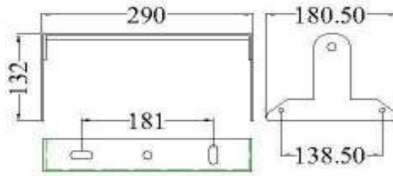
BatLED Brackets
